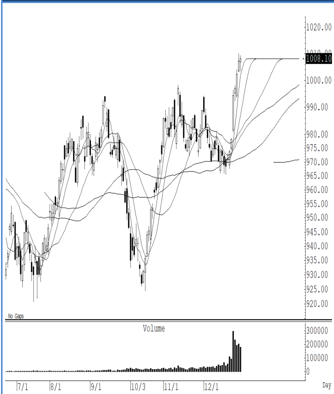
S50H23 (Close 1,008.10 Chg 0.80)
