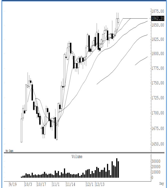
GOH23 (Close 1,862.20 Chg 0.50)
